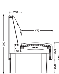
SECTION
