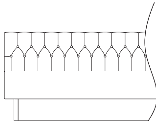
FRONT ELEVATION Typical Elevation
